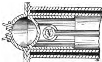
FIG. 292.—Section through a Gas Engine Cylinder having a spherical clearance and a spherical depression on the piston head. The shaded sections at top and bottom indicate the water jackets.
